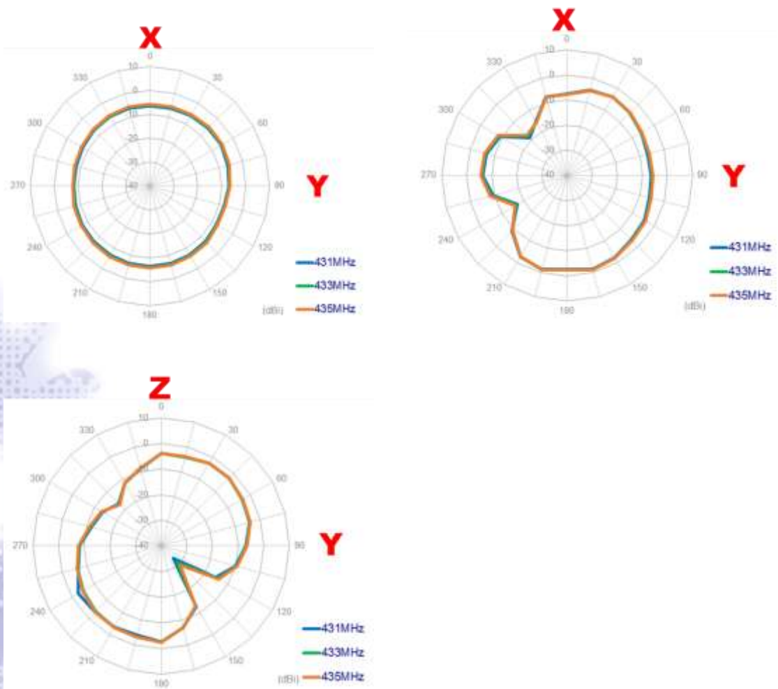
2D Radiation Pattern
